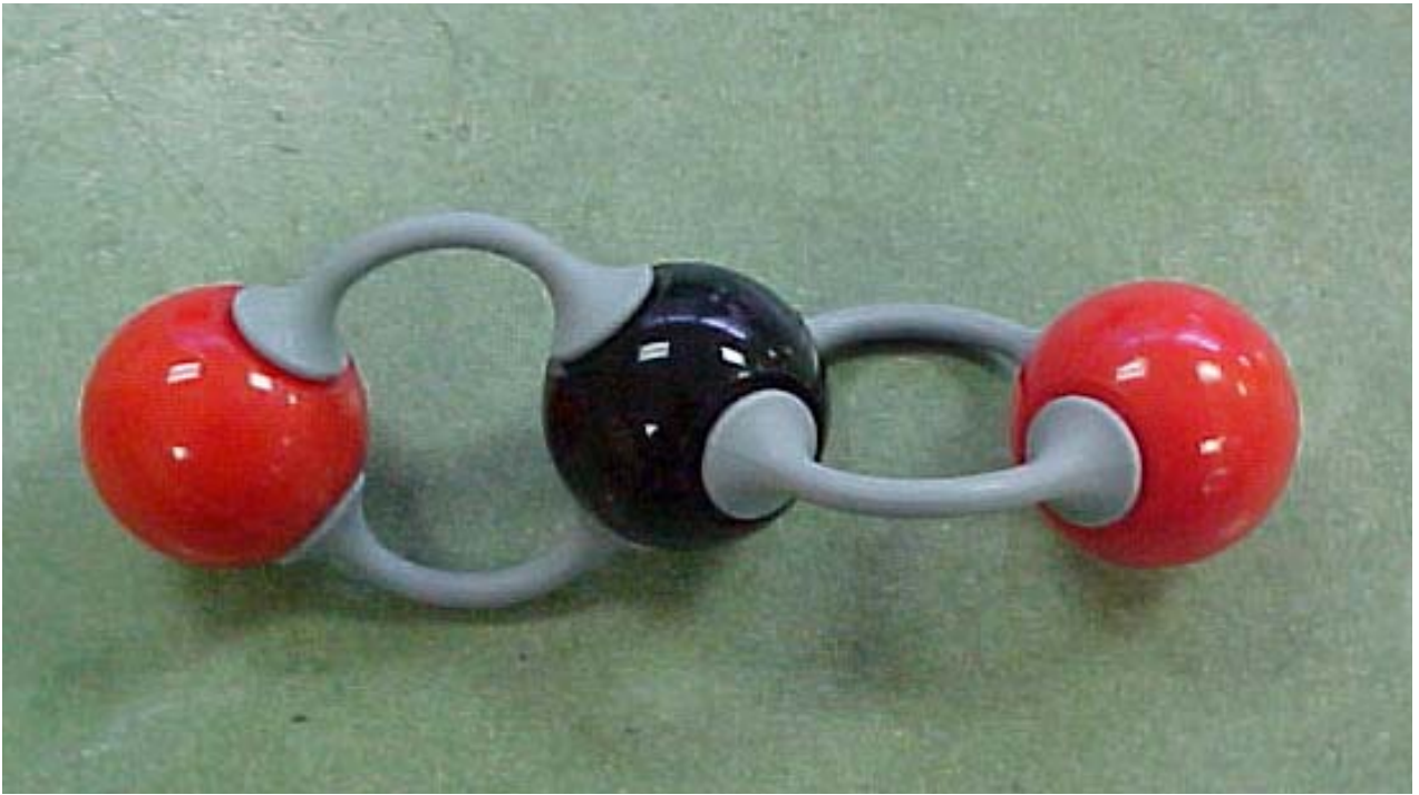
Carbon Dioxide
